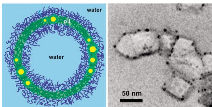
Fig. 1. (Left) Schematic illustration of the assembly of PEG-b-PLA polymersomes using water–oil–water double emulsion templates. The polymersomes are functionalized with dodecanethiol-stabilized gold nanoparticles. (Right) A transmission electron micrograph of the nanoparticle functionalized polymersomes.
