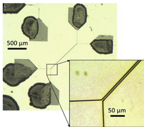
Fig. 2. Optical micrograph of 2 mm long, 5 \mu\text{m} wide double wires after filling two capillaries with Ag from two sides each. The thermoplastic polymer films were prepatterned by thermal NIL.
