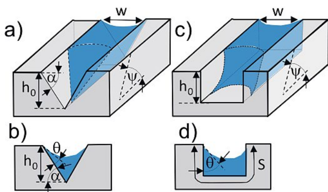
Fig. 1. Groove geometries and liquid spreading characteristics for a,b) V-grooves and c,d) U-grooves with flat bottom, with geometrical parameters width w , height h_0 and vertex angle \alpha , and wetting parameters \theta and \psi .
