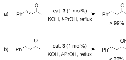
Scheme 3. Selective transfer hydrogenation of benzylideneacetone catalyzed with 3 gives exclusively benzylacetone, even though benzylacetone is converted to the fully saturated product in independent runs.
