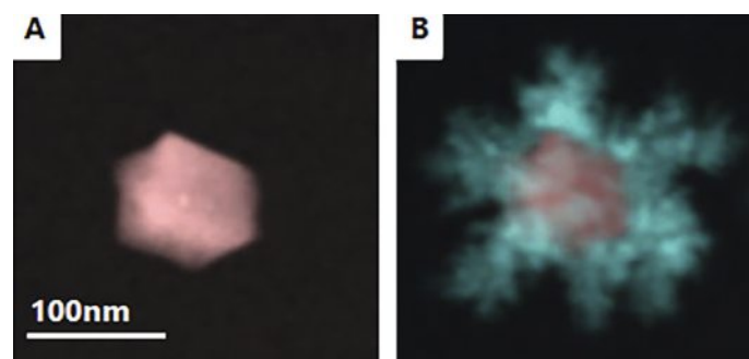
Fig. 2. Transition from reaction limited to diffusion limited growth. A) Annular dark-field scanning TEM image of a faceted Au nanostructure formed at an electron dose rate of 0.74 \text{ e}^-/\text{Å}^2\text{s} in 1 mM \text{HAuCl}_4 aqueous solution. B) At higher electron dose rate of 2.80 \text{ e}^-/\text{Å}^2\text{s} the growth mode changes to dendritic forming a shell over the faceted nanoparticle. [3]
