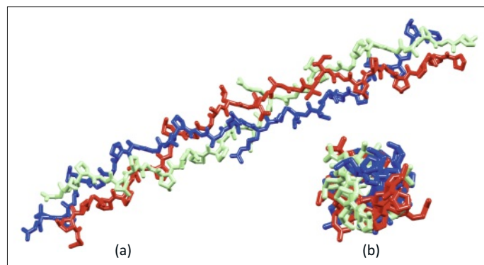
Fig. 4. Collagen is a fibrous protein. (a) The protein chains adopt helical conformations and three protein chains (shown in red, green and blue) combine to give a tube-like structure. (b) Looking down the tube-like collagen structure. [Data from the Protein Data Bank, PDB code 1BKV; \text{H}_2\text{O} molecules omitted.]
