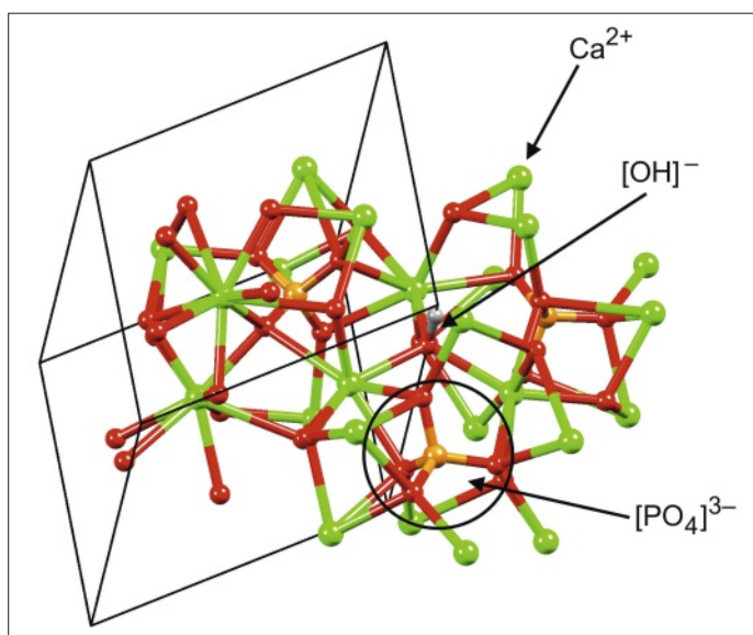
Fig. 3. The unit cell of hydroxyapatite with part of the 3-dimensional structure. \text{Ca}^{2+} ions are shown in green, the OH unit is directed along the crystallographic c -axis, and one [\text{PO}_4]^{3-} ion is highlighted (P, orange; O, red). [Data: R.T. Downs, M. Hall-Wallace, The American Mineralogist Crystal Structure Database , Amer. Mineral. 2003 , 88, 247.]
