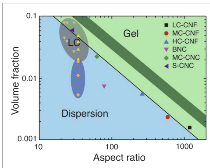
Fig. 1. Threshold volume fractions for the dispersion to gel transition for nanocellulose of varying type, charge and aspect ratios (adapted from ref. [2]). The data points within the shaded gray and blue areas represent compositions displaying liquid crystal (LC) ordering collected from ref. [3] (yellow triangles), ref. [4] (brown triangles) and ref. [5] (orange circles).
