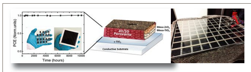
Fig. 1. Typical module stability test under 1 sun AM 1.5 G conditions for 10000 h. The device architecture with mixed 2D/3D perovskite. A picture of perovskite module size 100 X 120 cm developed at Soloronix SA, Aubonne.
