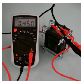
Small scale microbial fuel cell with multimeter, assembled by the participants in the workshop of Professor Fabian Fischer and used in experimental work. Photo Marc Sugnaux, HES-SO Valais.
