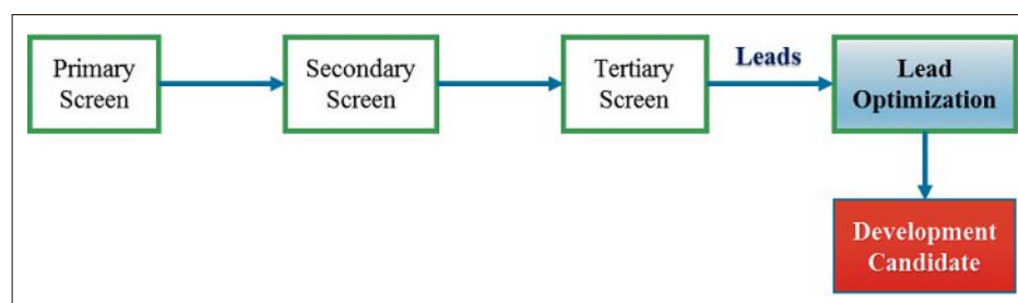
Fig. 6. Lead Optimisation, and selection of Development Candidate(s).
