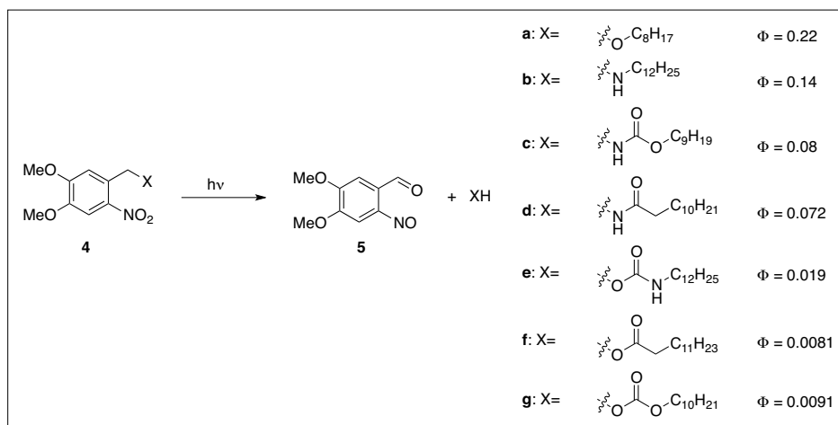
Scheme 2. Substituent effects on quantum yields.
