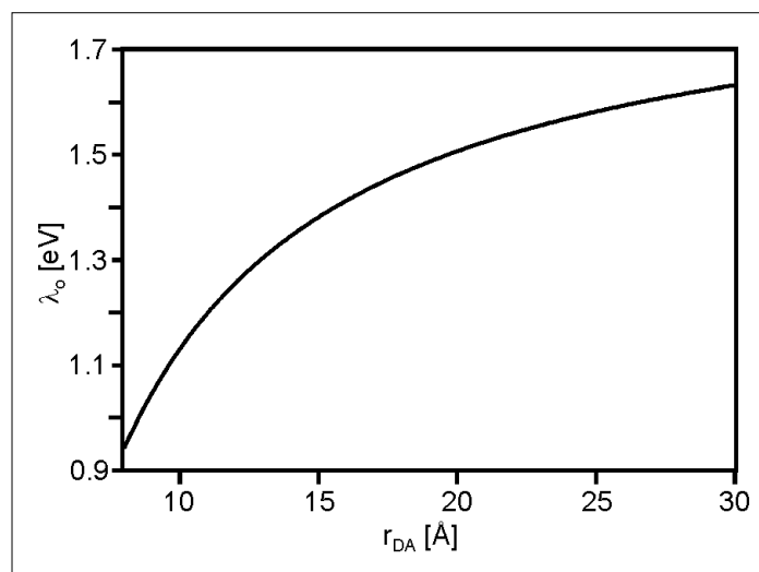
Fig. 2. Outer-sphere reorganization energy ( \lambda_o ) as a function donor–acceptor distance ( r_{\text{DA}} ) assuming spherical donors and acceptors with radii ( a_1, a_2 ) of 4 \text{ \AA} and \text{CH}_3\text{CN} ( \eta = 1.3341 , D_{\text{s}} = 35.7 ) as the solvent. Calculated using Eqn. (6).
