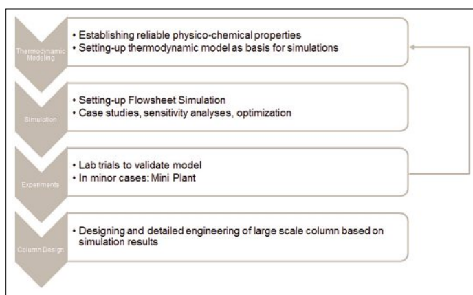
Fig. 2. Design procedure for dividing wall columns at Lonza.
