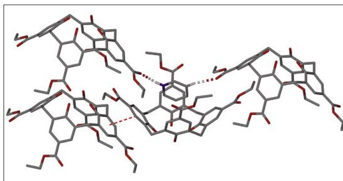
Fig. 2. Selectively labelled asymmetric unit in the single crystal X-ray structure of [\text{PyH}][\mathbf{3-H}] . Hydrogen bonding interactions are shown as split-colour dashed lines and \text{CH}\cdots\pi interactions are shown as red dashed lines. Hydrogen atoms (apart from those involved in hydrogen bonding and \text{CH}\cdots\pi interactions) omitted for clarity.
