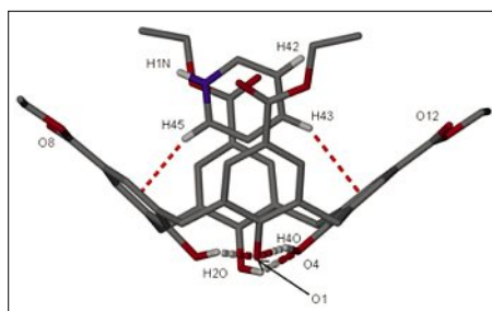
Fig. 2. Selectively labelled asymmetric unit in the single crystal X-ray structure of [\text{PyH}][\mathbf{3-H}] . Hydrogen bonding interactions are shown as split-colour dashed lines and \text{CH}\cdots\pi interactions are shown as red dashed lines. Hydrogen atoms (apart from those involved in hydrogen bonding and \text{CH}\cdots\pi interactions) omitted for clarity.
