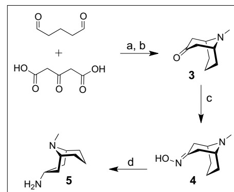
Scheme 2. Reagents and conditions: (a) \text{MeNH}_3\text{Cl} , \text{Na}_2\text{HPO}_4 , \text{NaOH} , 20 h, r.t.; (b) \text{HCl} , 1 h, 100 °C, for both steps: 95%; (c) \text{NaOAc} , \text{NH}_3\text{OHCl} , 4 h, r.t. 92%; (d) \text{H}_2\text{SO}_4 , \text{LiAlH}_4 , \text{THF} , 8 h, r.t. to 45 °C, 30–92%.
