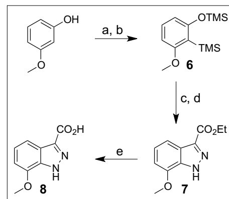
Scheme 4. Reagents and conditions: (a) \text{HMDS} , 1 h, 75 °C, crude; (b) i\text{-Pr}_2\text{NH} , n\text{-BuLi} , \text{TMS-Cl} , \text{THF} , 13 h, -78 °C to r.t., 87%; (c) n\text{-BuLi} , \text{Tf}_2\text{O} , \text{Et}_2\text{O} , 0 °C to r.t., 90%; (d) \text{N}_2\text{CHCO}_2\text{Et} , \text{TBAF} , \text{THF} , -78 °C to r.t., 24 h, 81%; (e) \text{NaOH} , \text{MeOH} , 14 h, 60 °C, quant.
