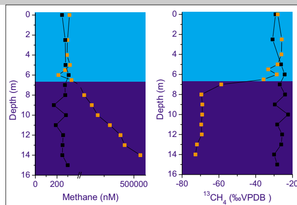
Methane concentration and isotopic composition profile of Rotsee in summer during stratification (orange dots) and in winter after the lake mixed (black dots).
