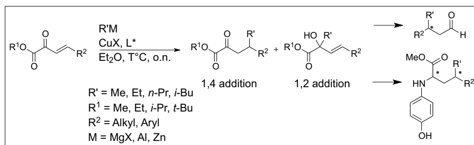
Scheme 1. Cu-catalyzed ACA to \beta,\gamma -unsaturated- \alpha -ketoesters.
