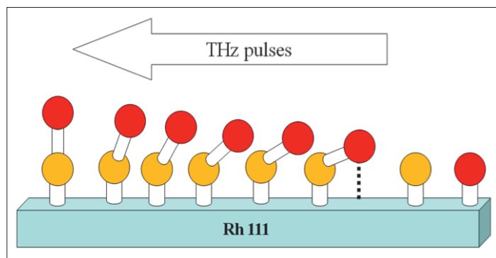
Fig. 1. A schematic representation of THz-induced dissociative absorption of CO (yellow = C, red = O) on a Rh surface.
