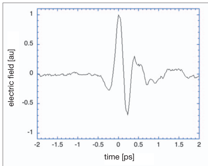
Fig. 2. An electro-optic sampling trace of the THz signal from the PSI optical rectification setup.
