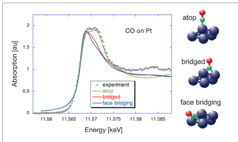
Fig. 3. A (static) near-edge X-ray absorption spectrum taken at the Pt edge at a synchrotron. [18] From the good match with theory, it is clear that the adsorbed CO is situated in the atop position.
