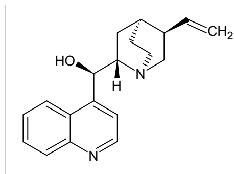
Fig. 1. Structure of the template molecule (–)-cinchonidine
