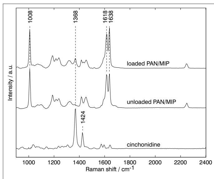
Fig. 4. Direct observation of target binding in a loaded MIP microsphere by a characteristic peak at 1368 cm -1 in the Raman spectra of a loaded (top) and an unloaded (middle) MAA/DVB-MIP electrospun into a PAN membrane. Bottom: Raman spectrum of the cinchonidine target molecule.
