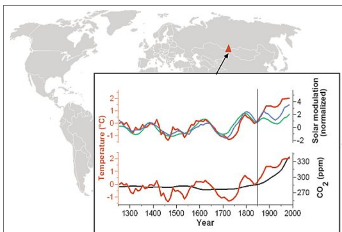
Location of the drilling site (triangle) and the Altai temperature reconstruction (red) compared with solar activity inferred from ^{10}\text{Be} (blue) and ^{14}\text{C} (green) and \text{CO}_2 concentration (black). The solar modulation curves were shifted by 20 years (average value of the lag between solar forcing and temperature response). The vertical line divides the pre-industrial era (1250–1850) from the last 150 years.
