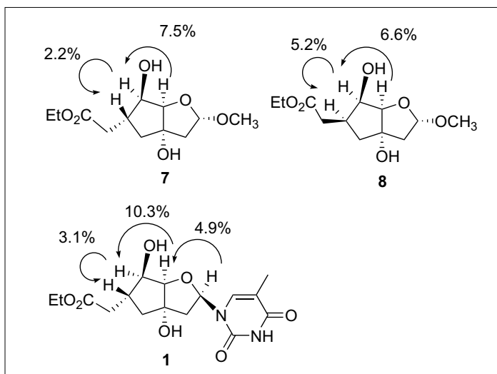
Fig. 2. Intensities of observed (mutual) ^1\text{H-NMR} difference NOE effects of the relevant protons used for assigning the cis - and trans -relationship of substituents in the carbocyclic ring in 7 and 8 as well as the \beta -anomeric configuration in 1
