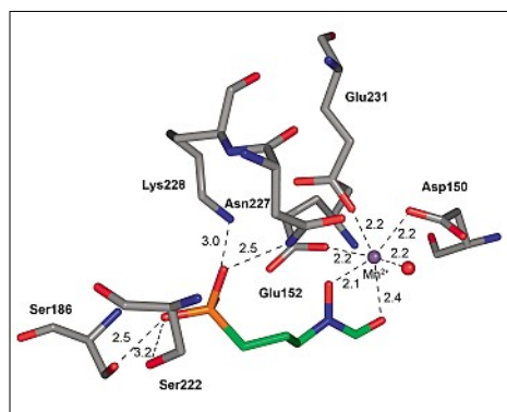
Fig. 3. Co-crystal structure of fosmidomycin and E. coli IspC (PDB code: IONP). [19] Color code: protein skeleton: C: gray; inhibitor skeleton: C: green; O: red; N: blue; P: orange; Mn 2+ : violet sphere, H 2 O: red sphere. Hydrogen-bond distances are given in Å.
