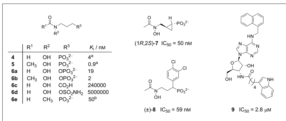
Fig. 2. Known inhibitors of IspC. [15-20] K_i = inhibition constant. Footnotes to Table: a K_i^* represents the conversion to the tightly bound complex, taking into account that fosmidomycin is a slow, tight-binding inhibitor. b The IC_{50} value is given as no K_i value has been published.
