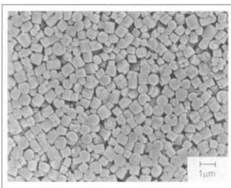
Fig. 2. SEM picture of a zeolite L sample.
