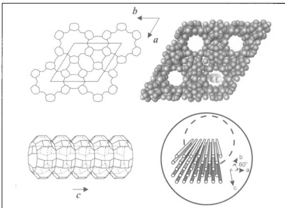
Fig. 3. Framework of zeolite L. Upper: top view, perpendicular to the c -axis, displayed as stick- (left) and as Van der Waals- (right) representation with a dye molecule entering the zeolite channel. Lower: Side view of a channel along the c -axis, without bridging oxygen atoms (left). Schematic view of some channels in a hexagonal zeolite crystal with cylinder morphology.
