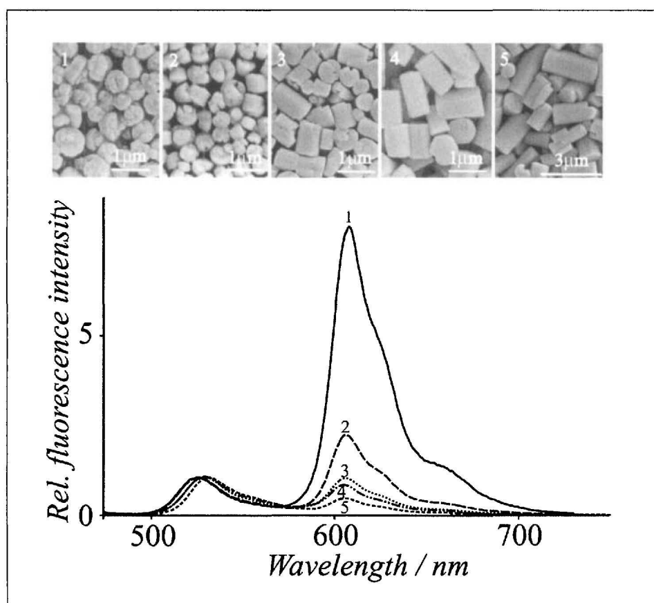
Fig. 4. Upper: SEM pictures of the investigated zeolite L samples with different crystal length: 1, 300 nm; 2, 500 nm; 3, 850 nm; 4, 1400 nm; 5, 2400 nm. Lower: Fluorescence intensity, after specific excitation of only \text{Py}^+ at 460 nm (scaled to the same height at the maximum of the \text{Py}^+ emission) of \text{Py}^+ loaded and \text{Ox}^+ modified zeolite L crystals with constant \text{Py}^+ loading, for different crystal lengths. The \text{Ox}^+ modification was two molecules at both ends of the channel, on average.
