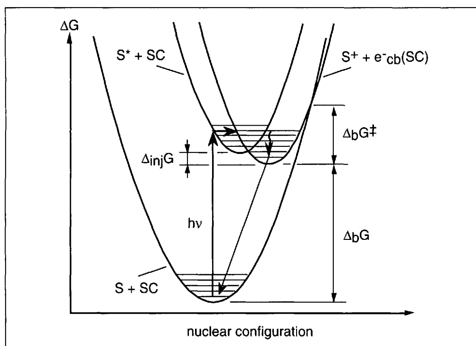
Fig. 1. Conceptual drawing showing free-energy surface crossing for interfacial charge-transfer processes depicted by Eqns. 2 and 3. While electron injection is kinetically nearly optimum ( \Delta G^\ddagger \approx 0 ), charge recombination falls deep into the inverted region. In the latter case, nuclear tunneling is likely to occur predominately, due to efficient contribution of the high-frequency vibrational modes and important Frank-Condon overlap.
