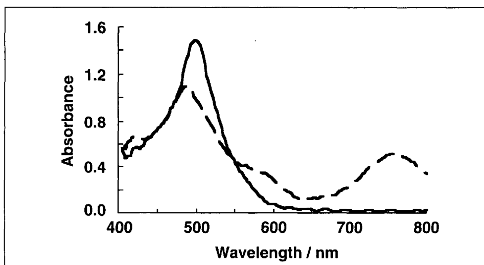
Fig. 2. Absorption spectra of the \text{TiO}_2 -supported diad 1 in the dark (dotted line) and under white light illumination (solid line). Electrode was polarized in both cases at +0.55 V vs. NHE.
