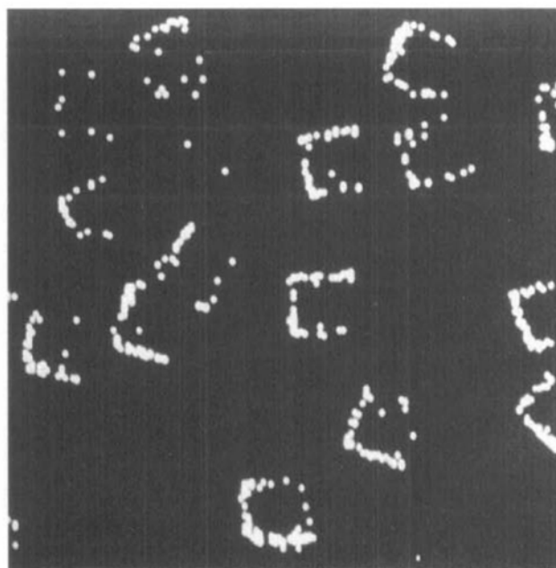
Fig. 5. Imaging SIMS iodide picture of AgBr microcrystals containing 0.13 mol-% iodide. An iodide ring is predominantly formed along edges and corners of the cubic AgBr crystals (1.24- \mu\text{m} edge-length).
